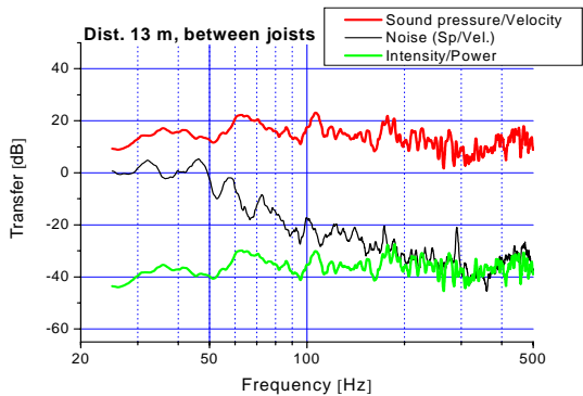
Figure 14. Transfer functions with microphone 13 m away from the excitation point.
