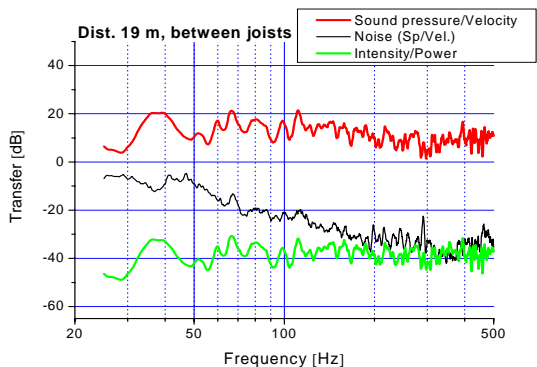
Figure 15. Transfer functions with microphone 19 m away from the excitation point.
