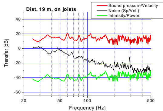
Figure 19. Transfer functions with microphone 19 m away from the excitation point.
