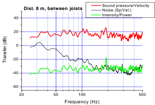
Figure 13. Transfer functions with microphone 8 m away from the excitation point.
