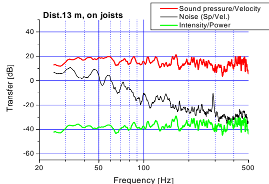
Figure 18. Transfer functions with microphone 13 m away from the excitation point.
