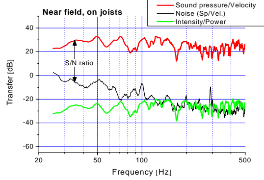
Figure 16. Near-field transfer functions.
