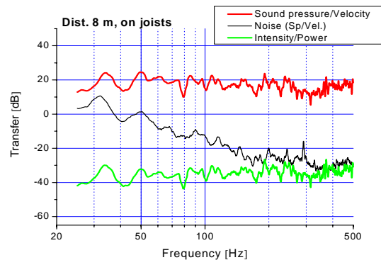
Figure 17. Transfer functions with microphone 8 m away from the excitation point.
