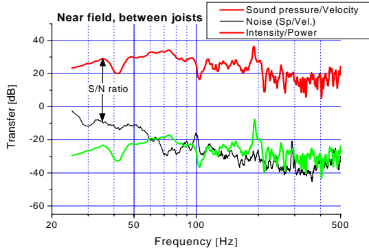
Figure 12. Near-field transfer functions.
